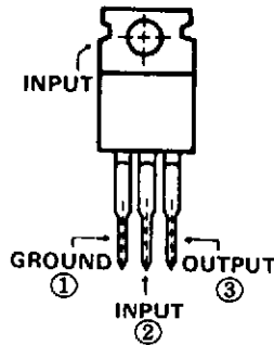
1. Package Outline
